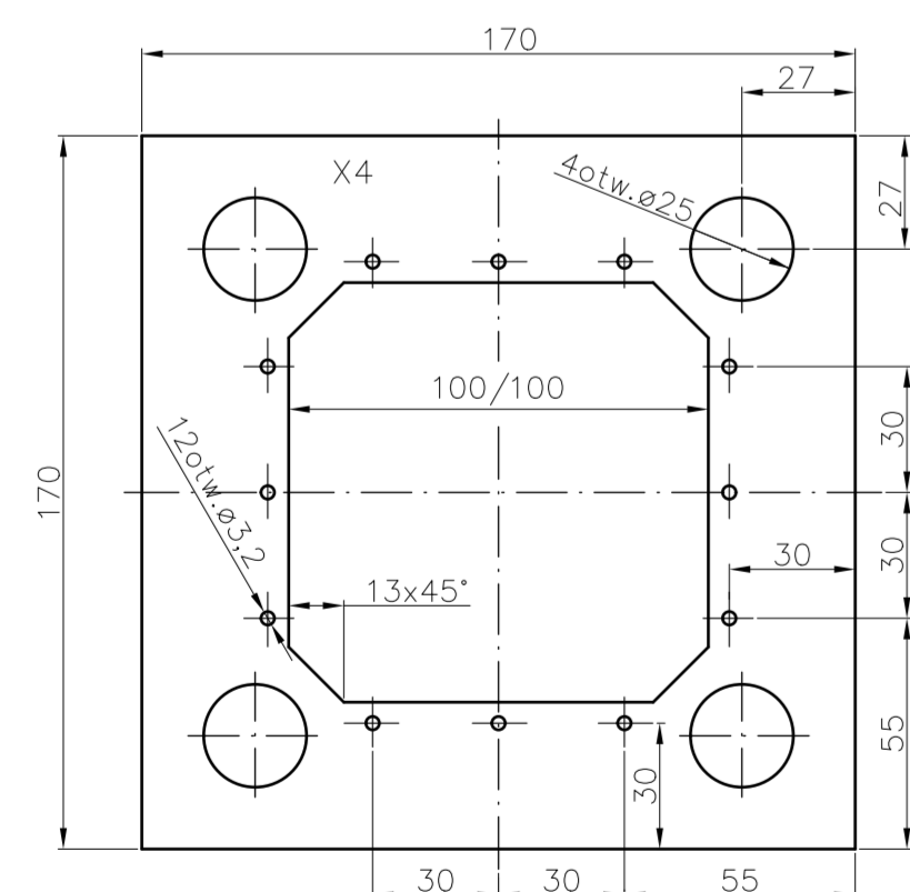
Rys.673/71
